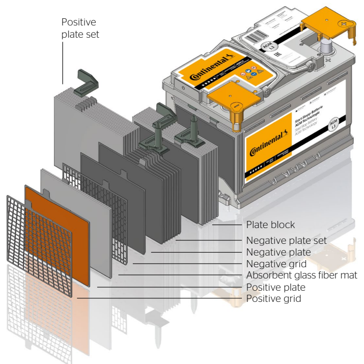
AGM technology: Battery construction
